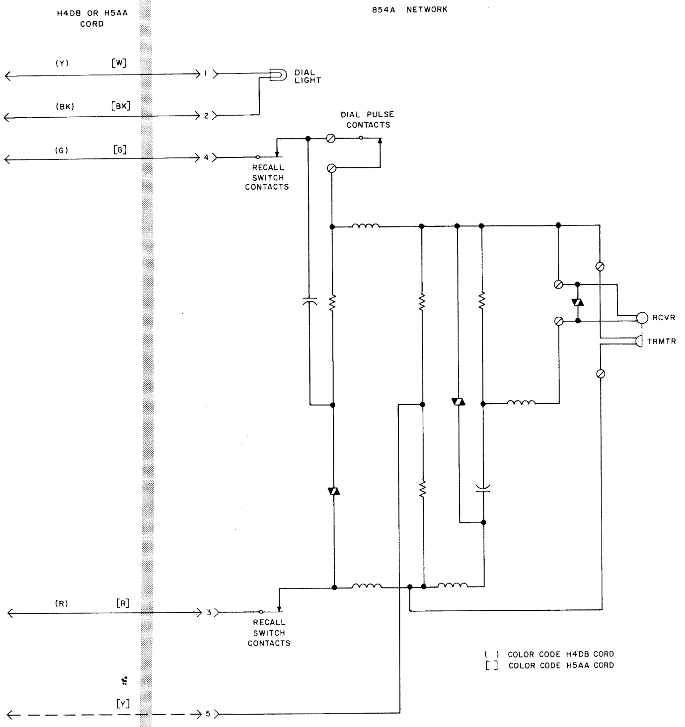
Fig. 11—220A Hand Telephone Set—Wiring Diagram
